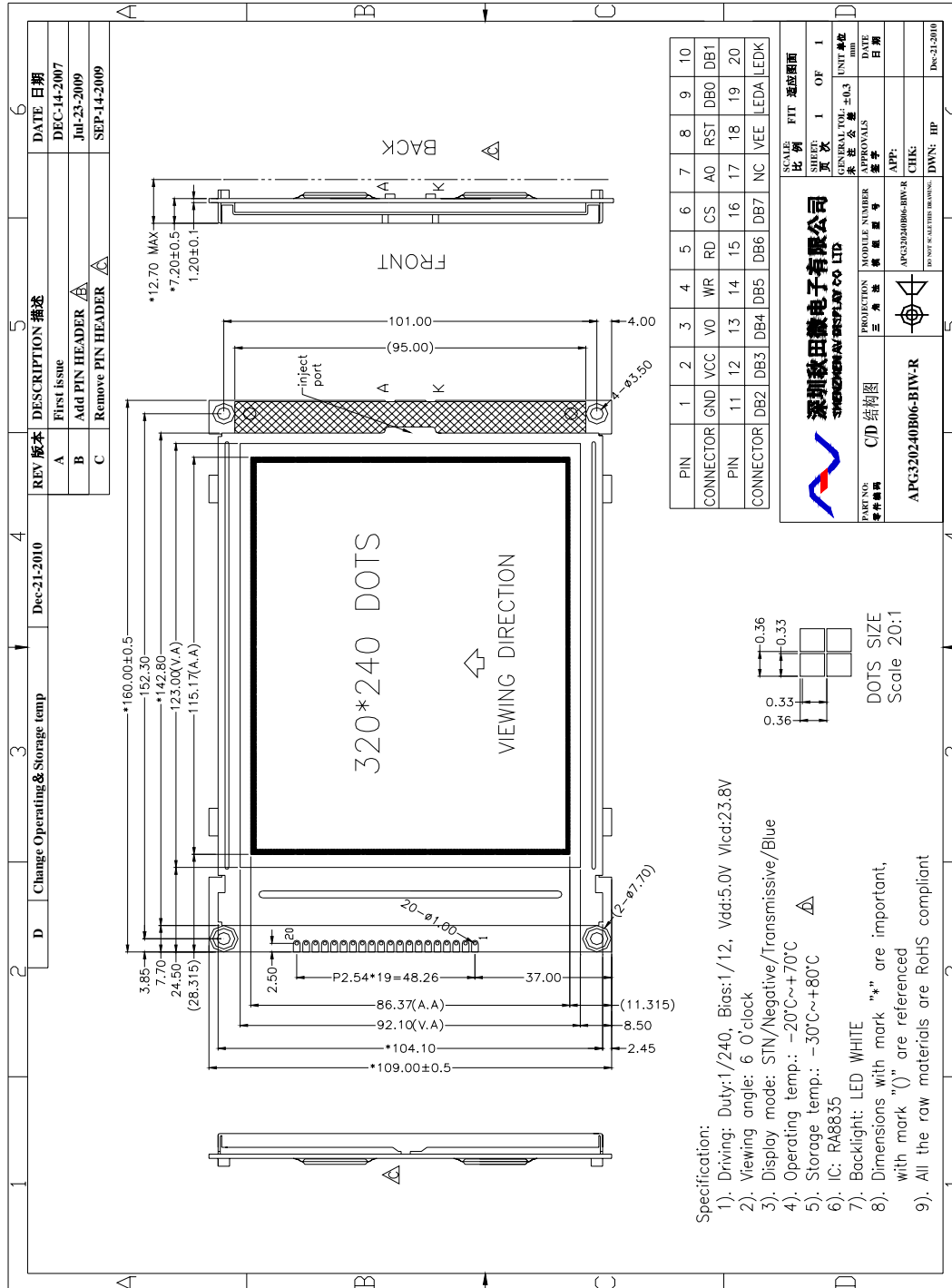
Figure 2. Dimensional outline
